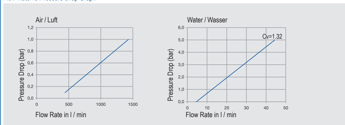
Flow Rate vs Pressure Drop Graph
